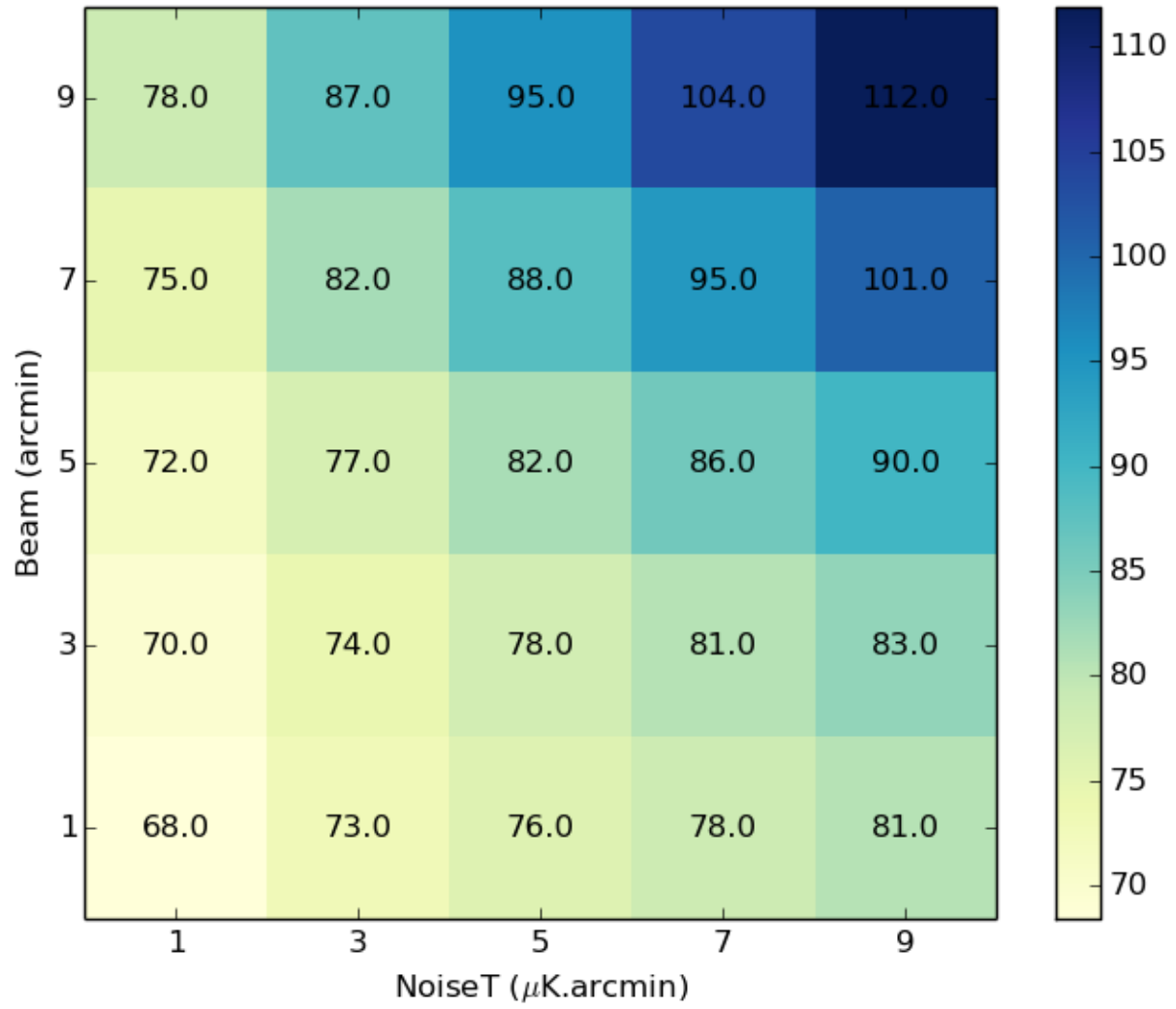
Constraint on neutrino mass
